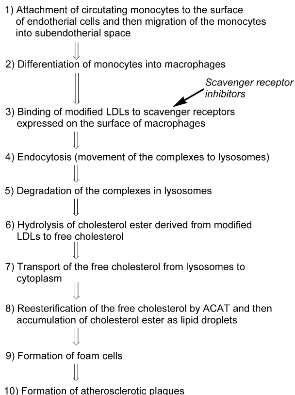
Figure 1. Schematic progress of atherosclerosis.
