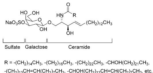
Figure 2. Structure of sulfatides.
