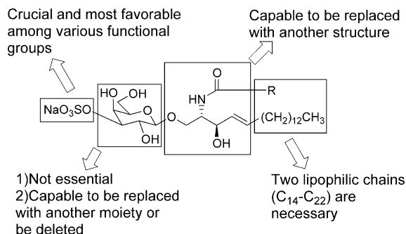
Figure 3. SARs of sulfatides.
